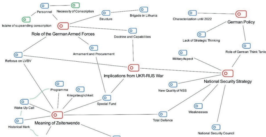
Figure 1 – Interview Codes Source: Author (2024) based on Analyse Tool MAXQDA.
